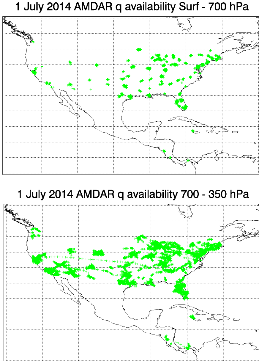
Figure 4. Coverage of AMDAR water vapour profile data over the US for 1 July 2014 at high (lower panel) and low levels (top panel)
